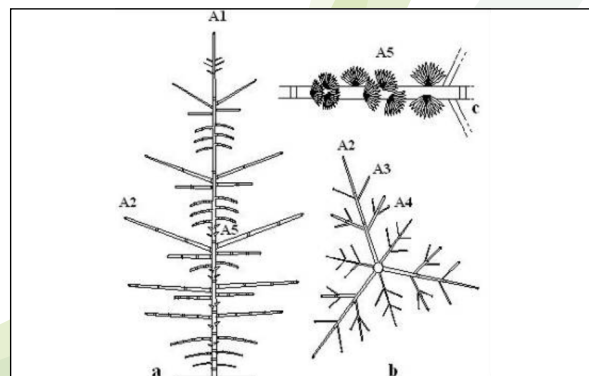
Figure 1: Architectural unit for Cedrus atlantica (A1: Main stem, A2: Branches, A3: Twigs, A4: Fine twigs, A5: Annual shoots).
