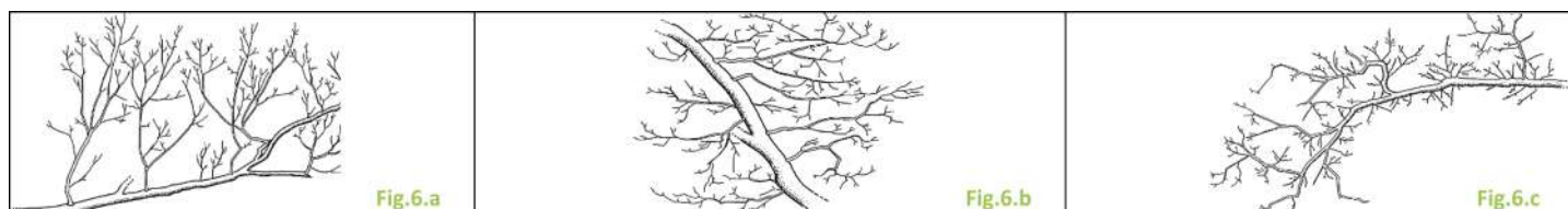
Figure 6: Graphical example of substitutes: orthotropic (Fig. 6.a), plagiotropic (Fig. 6.b) and ageotropic (Fig. 6.c).
